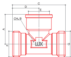
RT 908 Raccordo a T FxMxM.
